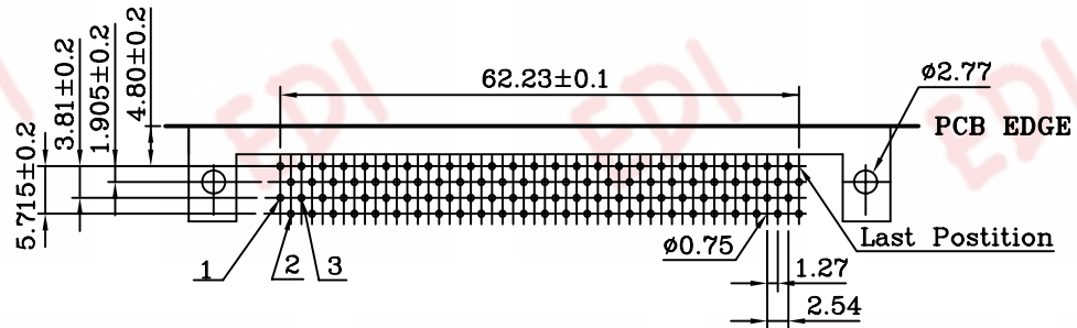
PCB LAYOUT
